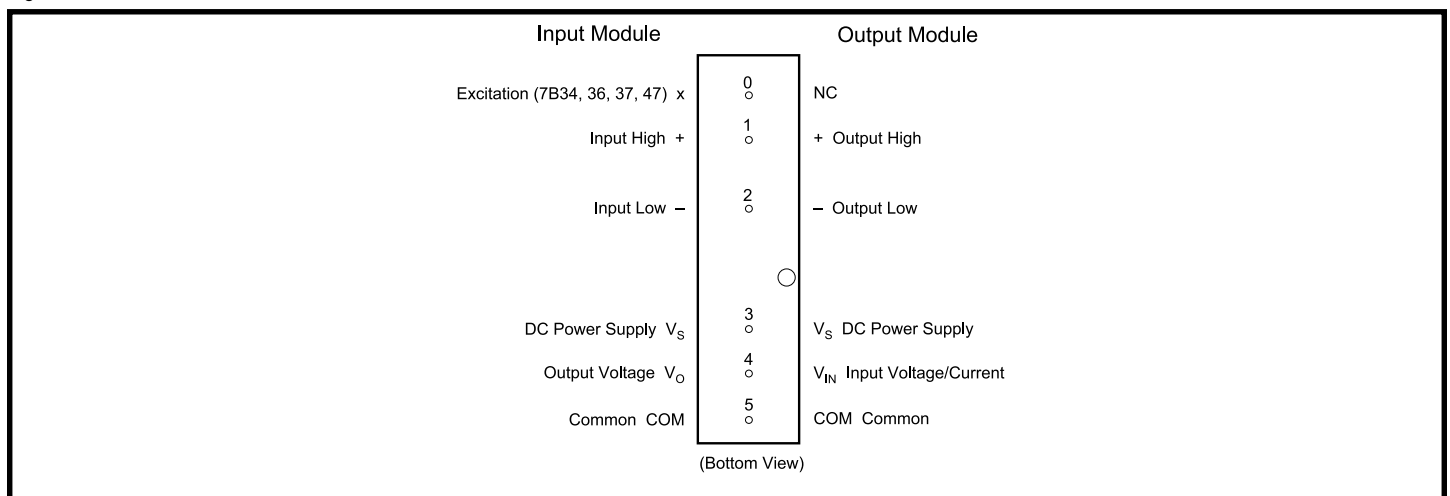
Figure 2: SCM7B Pinouts
