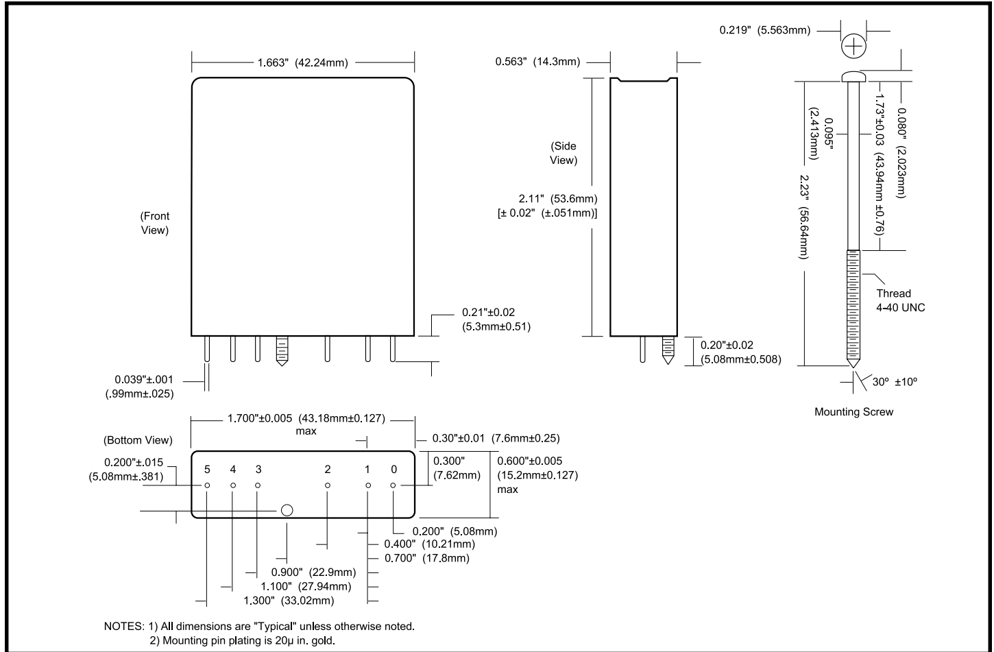
Figure 1: SCM7B Module Dimensions
