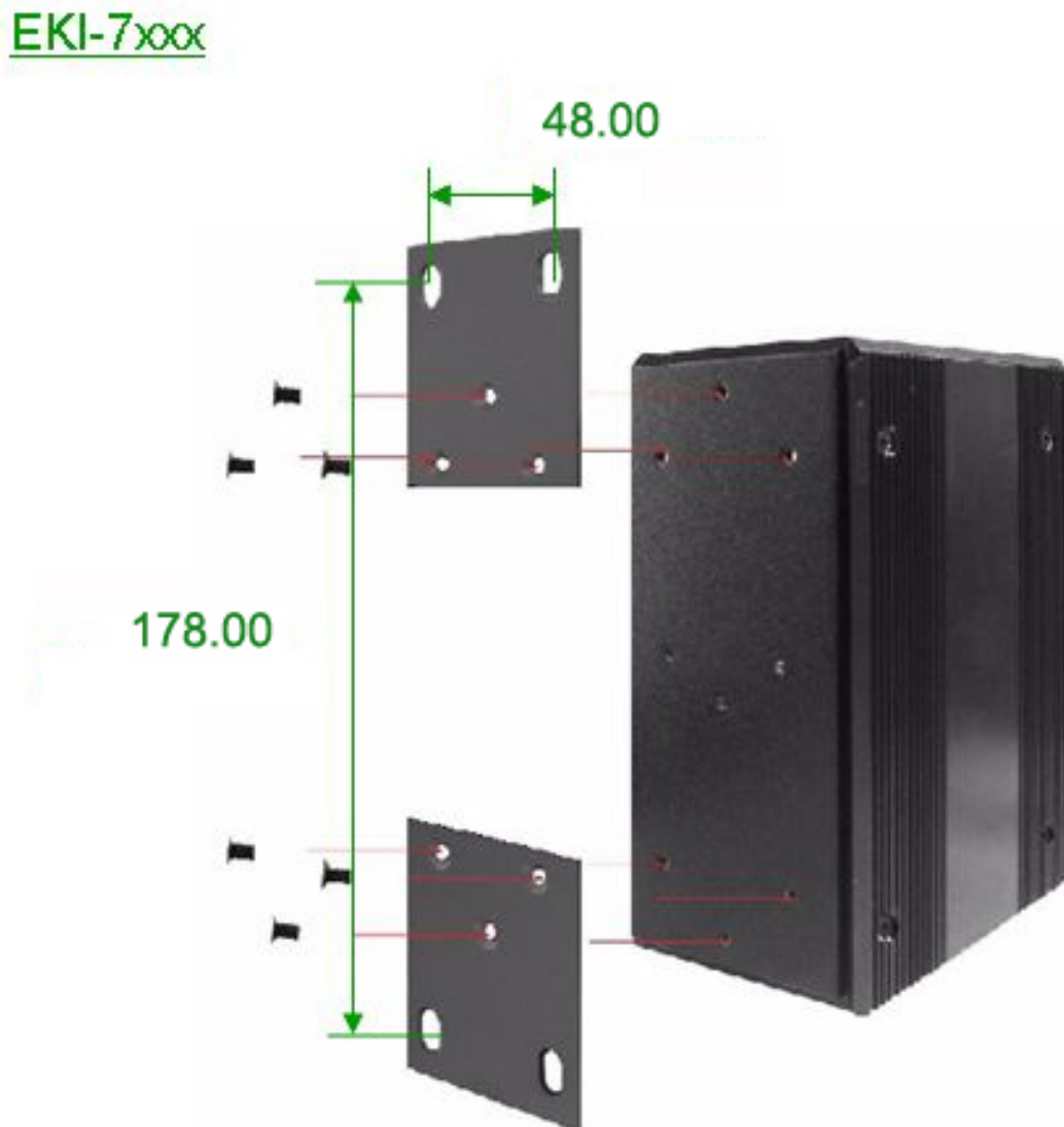
Figure 2.5: Combine the Metal Mounting Kit (units: mm)
