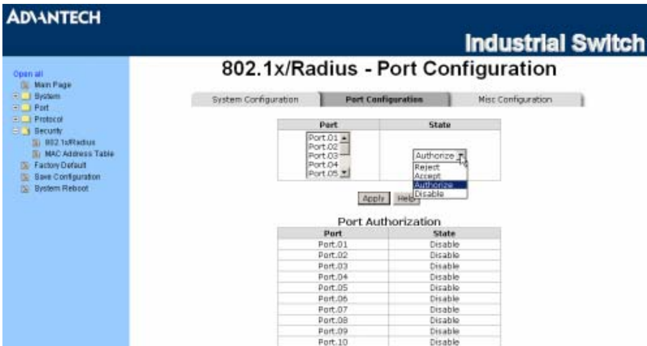
Figure 3.49: 802.1x/RADIUS - Port Setting interface
