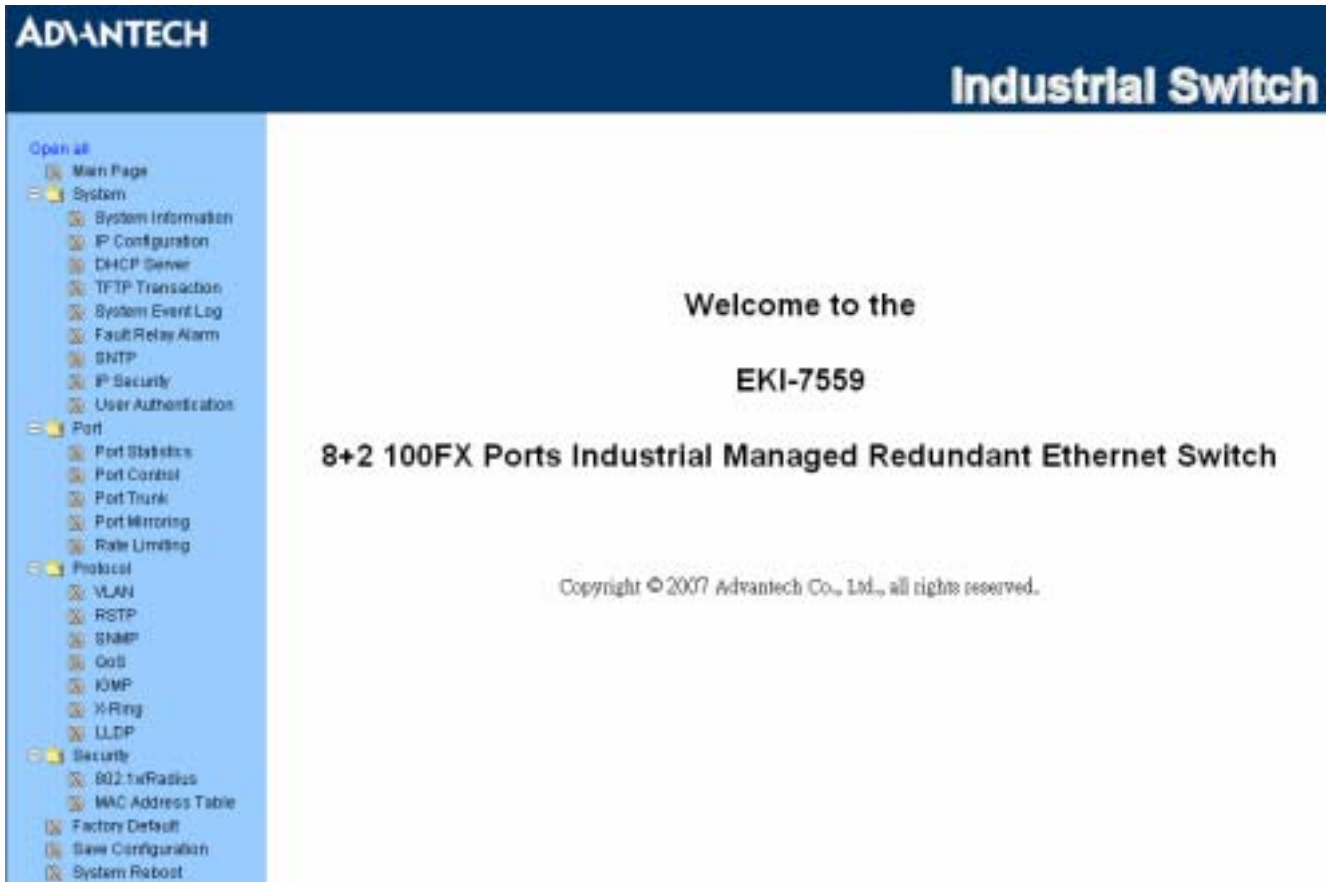
Figure 3.7: Main page
