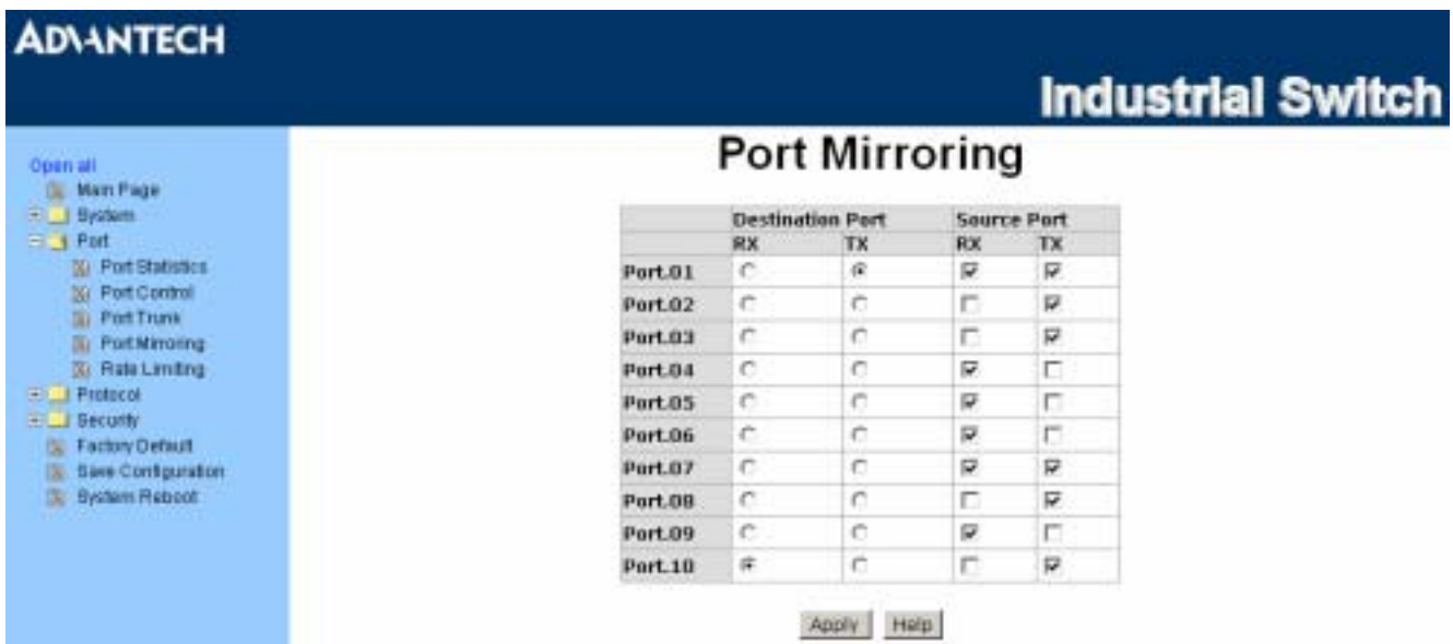
Figure 3.30: Port Mirroring
