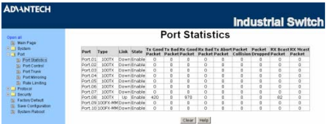
Figure 3.23: Port Statistics
