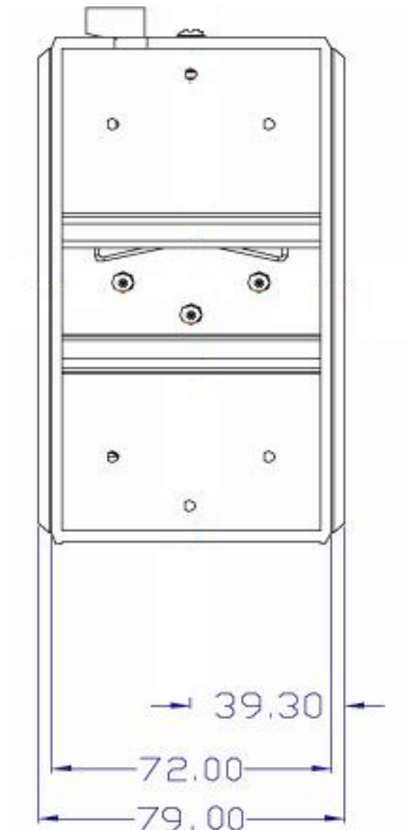
Figure 2.3: Rear View of EKI-7559MI/SI
