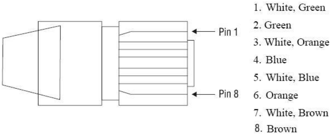
Figure A.3: EIA/TIA-568A
