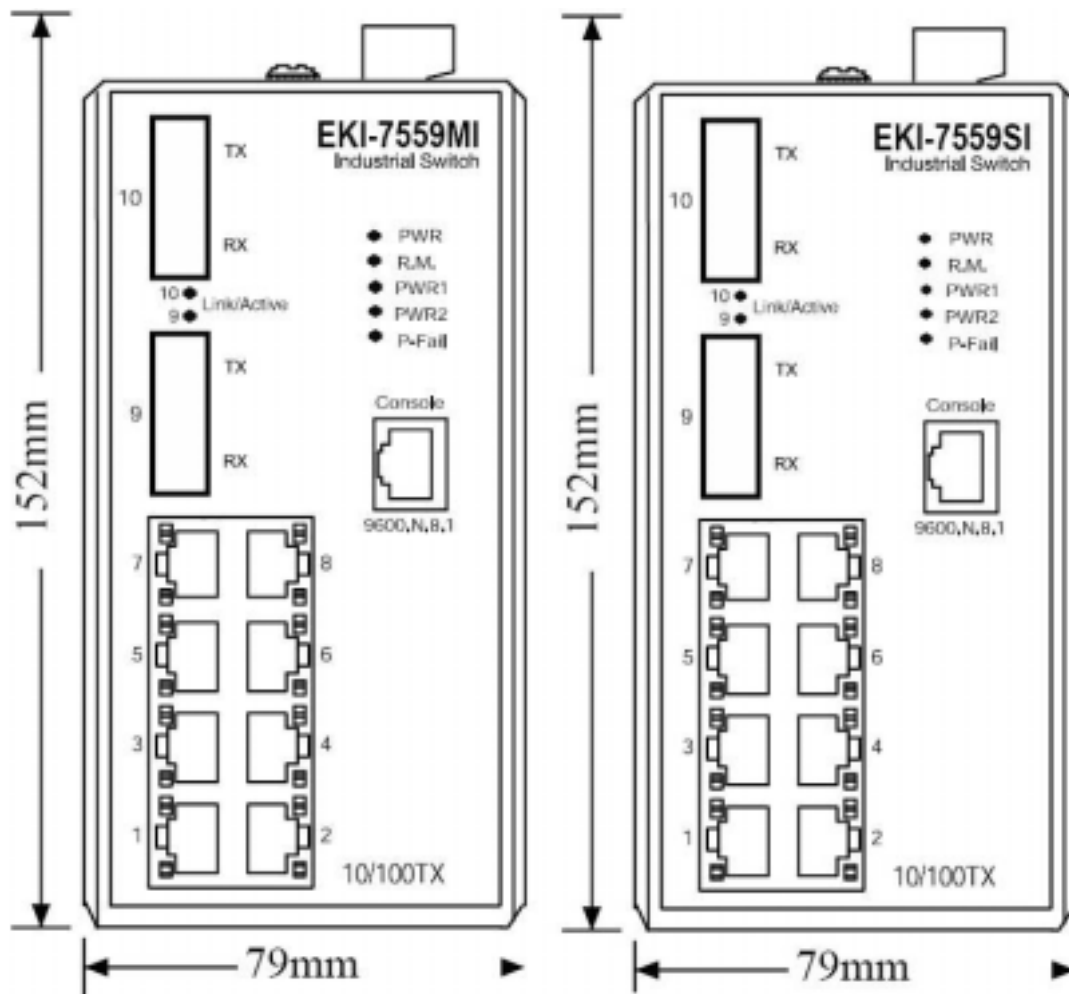
Figure 2.1: Front View of EKI-7559MI/SI
