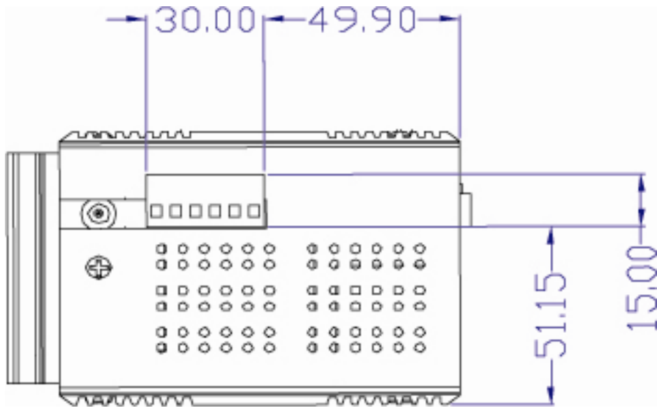
Figure 2.4: Top View of EKI-7559MI/SI
