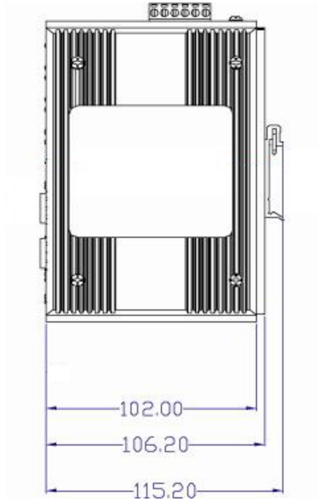
Figure 2.2: Side View of EKI-7559MI/SI
