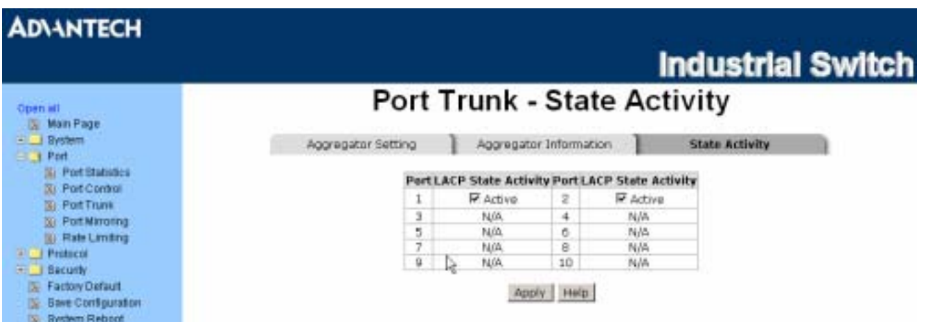
Figure 3.29: State Activity
