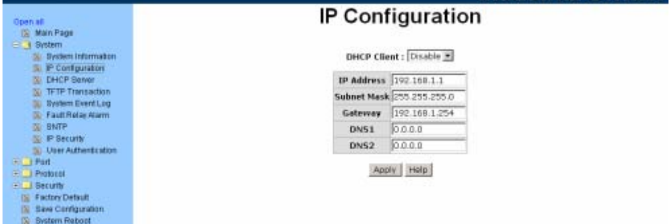
Figure 3.9: IP Configuration
