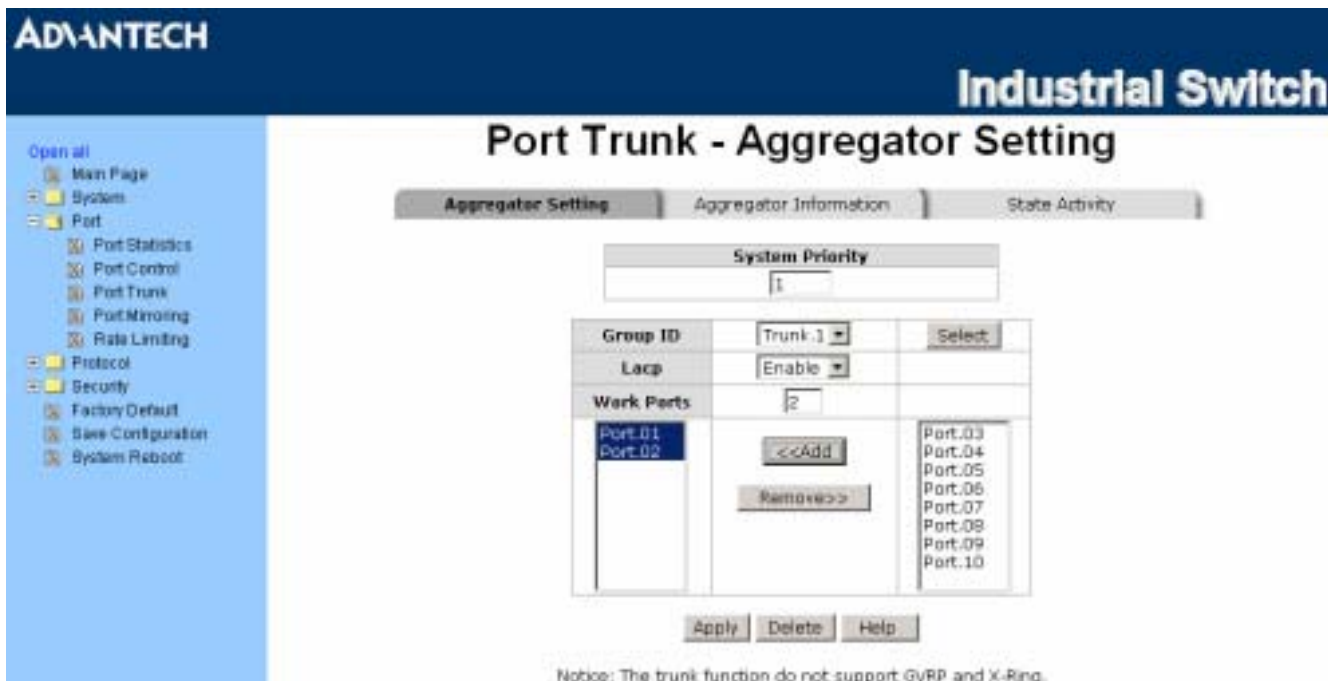
Figure 3.25: Aggregator Setting
