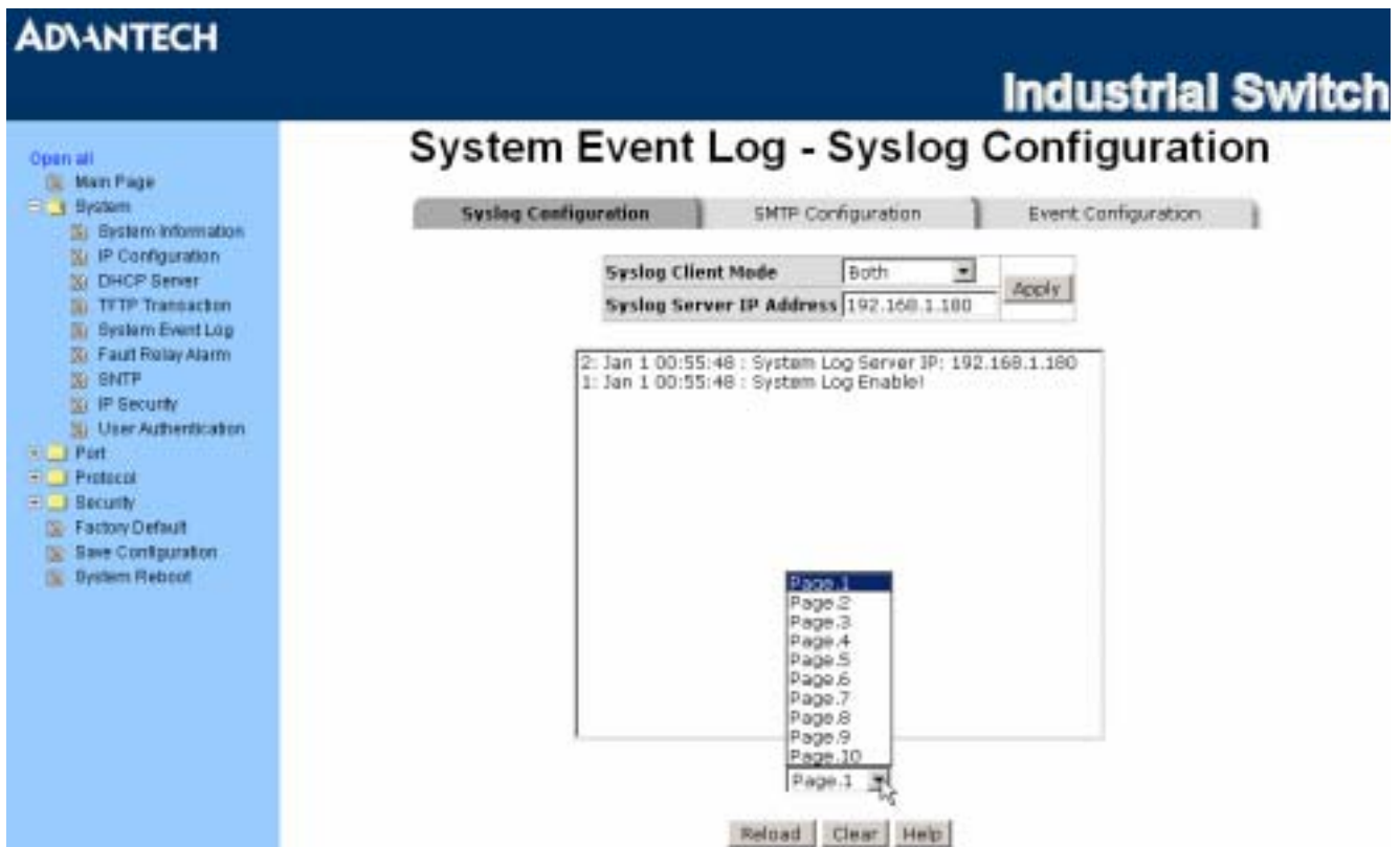
Figure 3.16: Syslog Configuration
