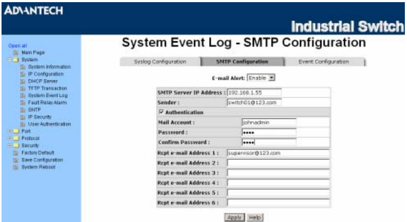
Figure 3.17: SMTP Configuration
