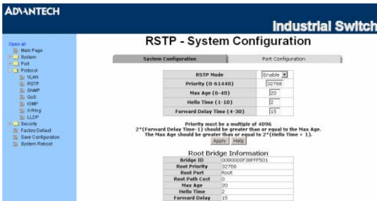
Figure 3.39: RSTP System Configuration interface
