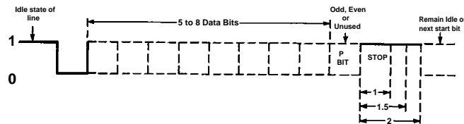
Figure 3: Asynchronous Bit Diagram
